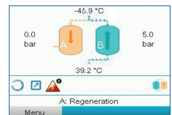
HMI Controller
